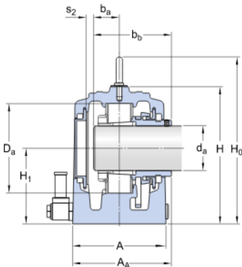
Split plummer block housings
